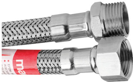
Nickle Plated Brass Fitting EPDM, PEX Tube
